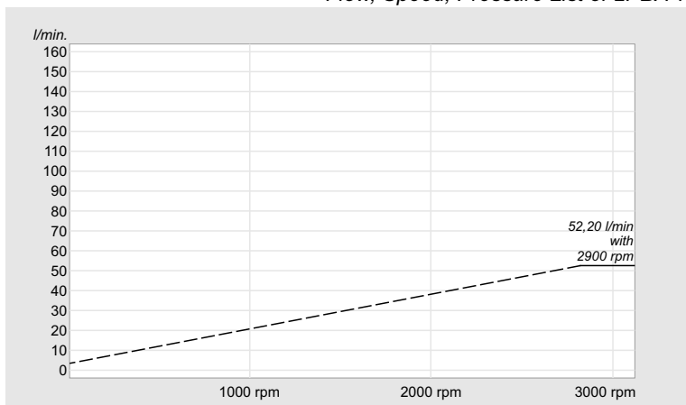
Flow, Speed, Pressure List of 2PBA 18
